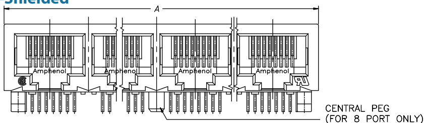
FRONT VIEW
