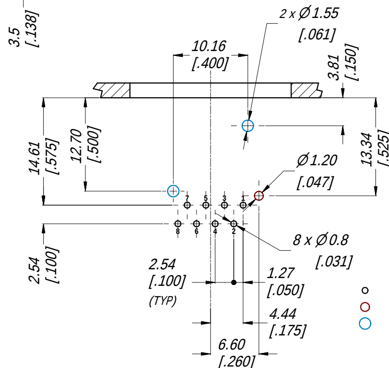
PCB LAYOUT 2:1 (CONNECTOR TOP VIEW)
