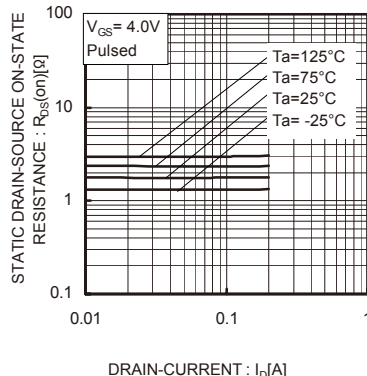
Fig.5 Static Drain-Source On-State Resistance vs. Drain Current(III)
