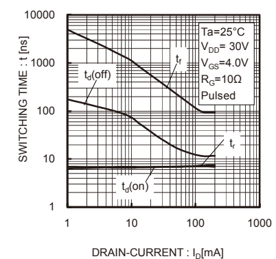
Fig.9 Switching Characteristics
