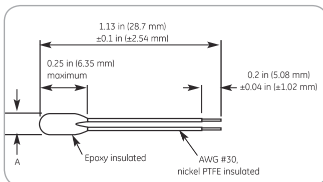
NTC Type MS Dimensions
