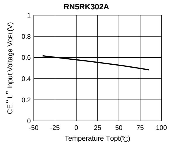
14) CE “L” Input Voltage vs. Temperature
