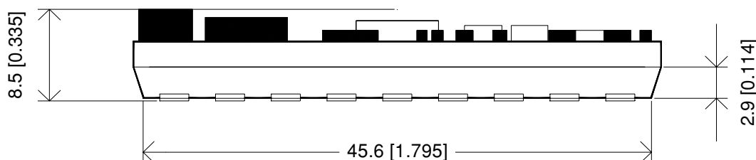
Height Profile
