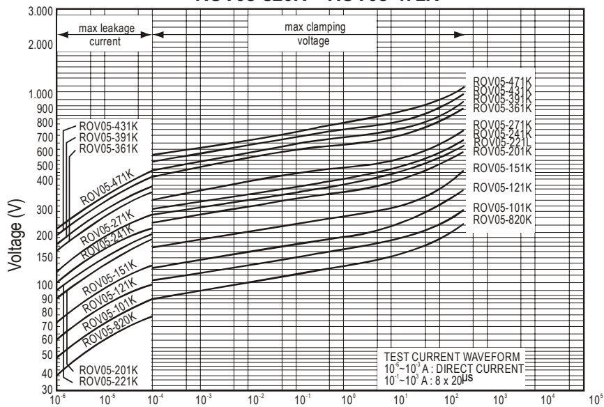
ROV05-820K – ROV05-471K
