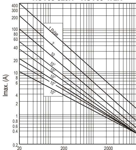
ROV05-820K – ROV05-471K
