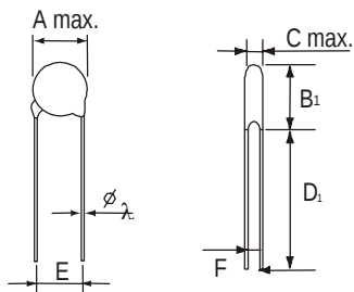
STRAIGHT LEAD TYPE (-S) Table of C max., F, and B₁ max.
