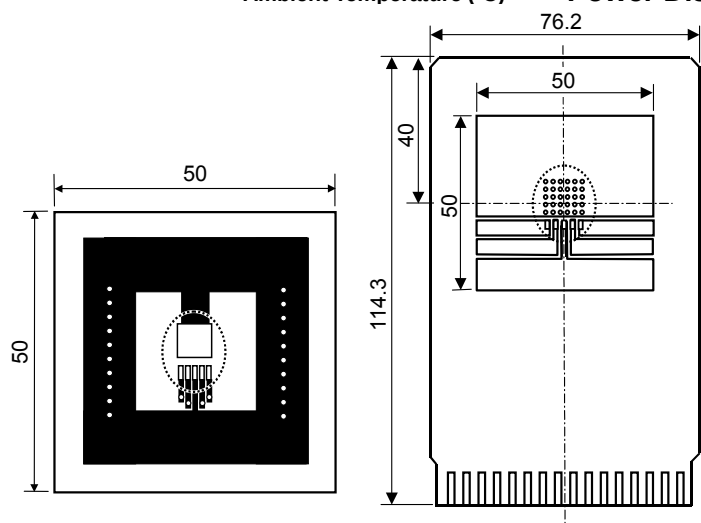
Standard Land Pattern
