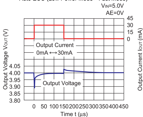
RP201x40xx Auto ECO (Low Power Mode ↔ Fast Mode)
