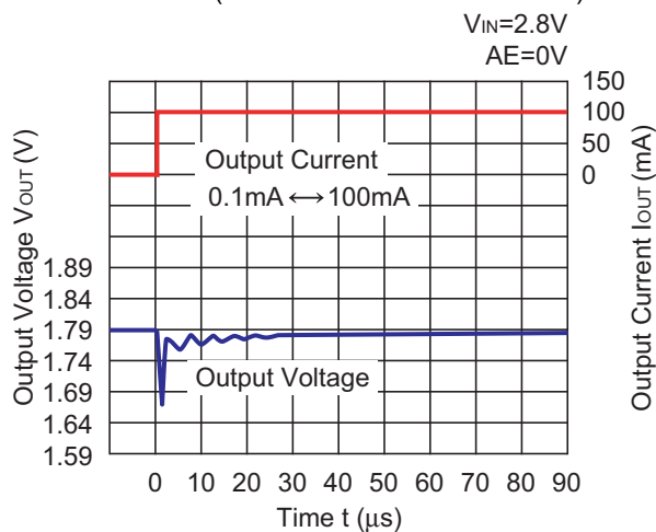
RP201x18xx Auto ECO (Low Power Mode \rightarrow Fast Mode)
