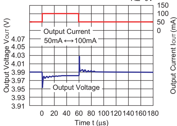
RP201x40xx (Auto ECO Fast Mode)
