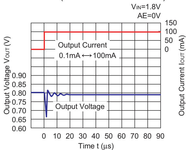
RP201x08xx Auto ECO (Low Power Mode \rightarrow Fast Mode)
