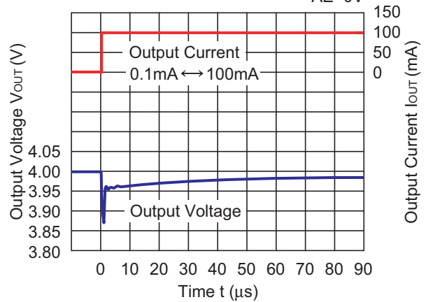
RP200x40xx Auto ECO (Low Power Mode→Fast Mode) V_{IN}=5.0V AE=0V
