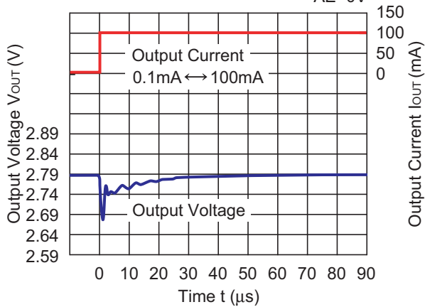
RP200x28xx Auto ECO (Low Power Mode→Fast Mode) V_{IN}=3.8V AE=0V
