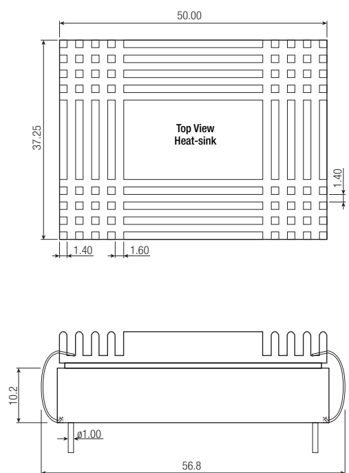
Dimension Drawing (mm) with Heat-sink
