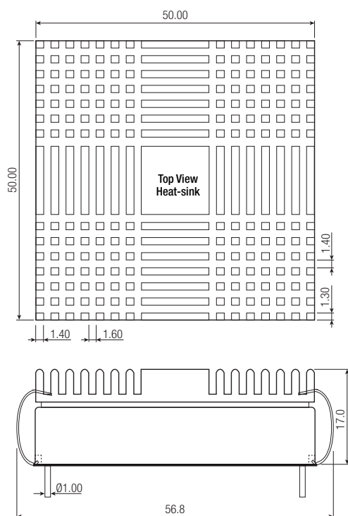
Dimension Drawing (mm) with Heat-sink
