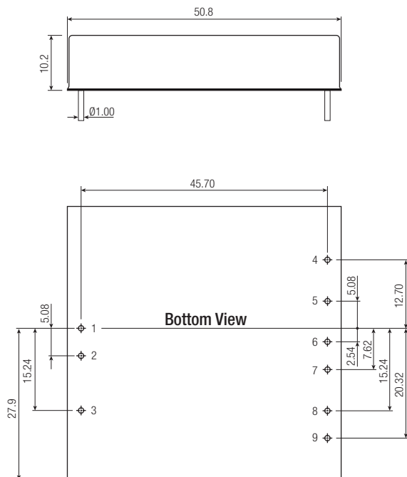
Dimension Drawing (mm)
