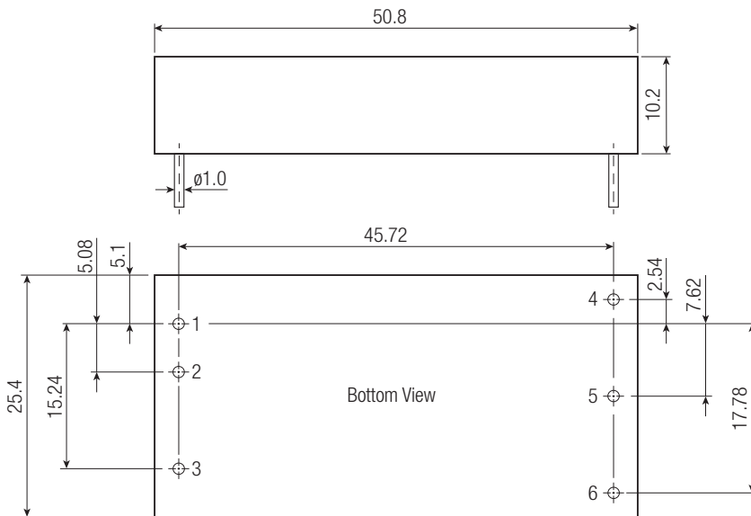
Dimension Drawing with Heat-sink (mm)
