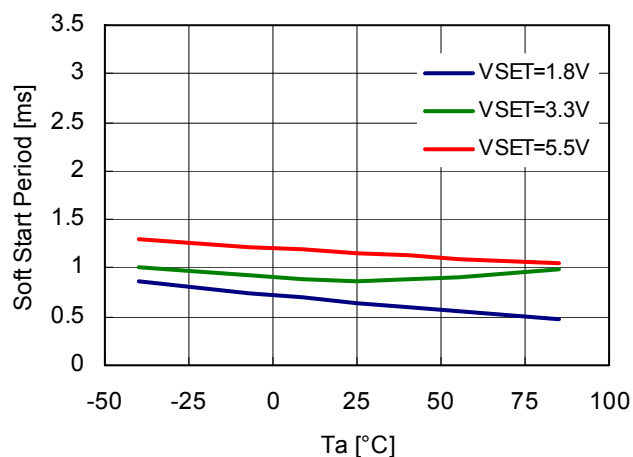
Soft Start Period vs. Temperature RP401xxx1x
