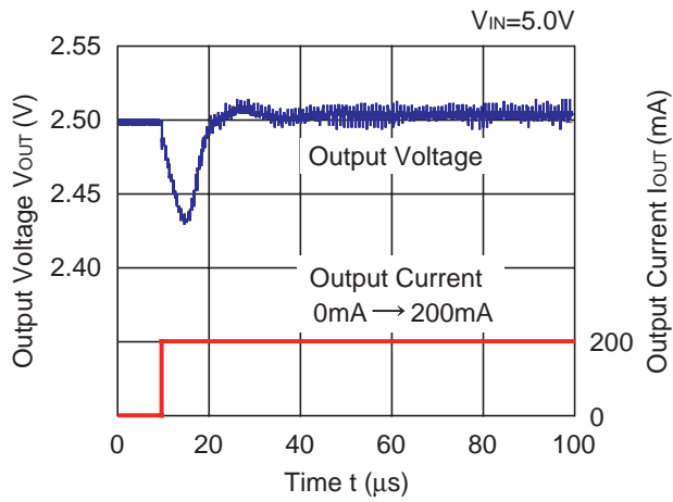
RP500x251A/253A
