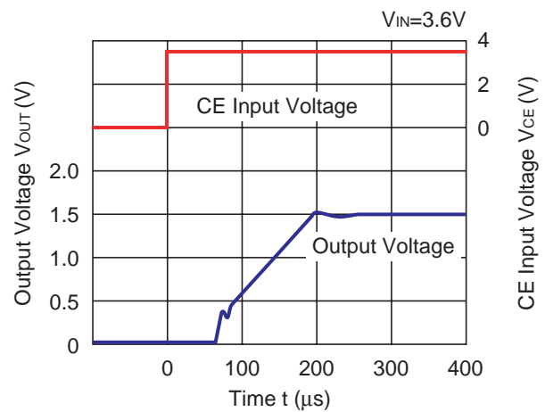
RP500x152A/154A ( I_{OUT}=1.5\text{mA} )
