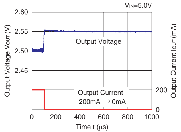
RP500x251A/253A
