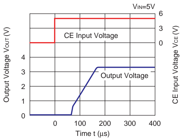
RP500x331A/333A ( I_{OUT}=3.3\text{mA} )
