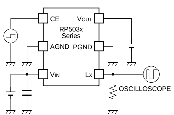
Soft-start Time
