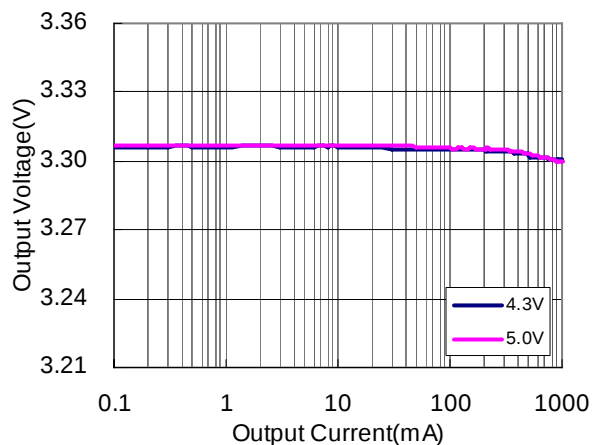
RP501K331x(PWM fixed)
