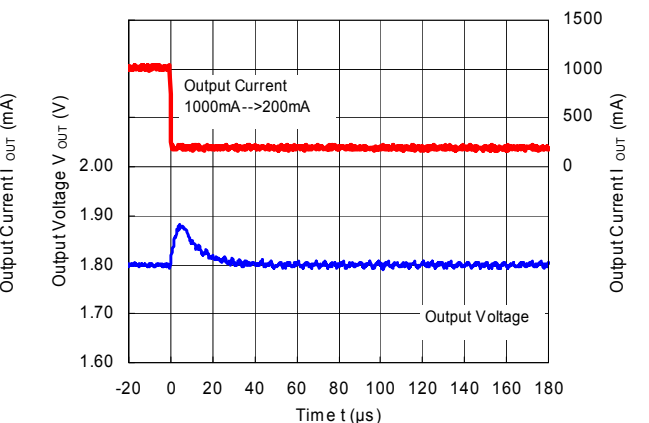
RP506Kxx1A/B/C ( V_{IN} = 3.6\text{ V} , V_{OUT} = 1.8\text{ V} ) MODE = "L" PWM/VFM Auto Switching Control
