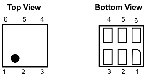
DFN(PLP)1212-6F Pin Configurations
