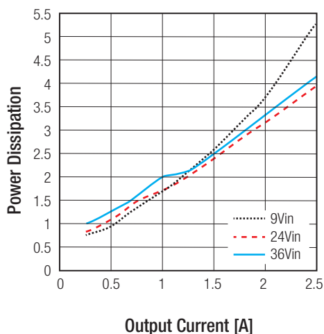
Power Dissipation vs Output Current
