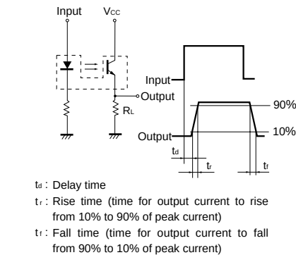
Fig.11 Response time measurement circuit
