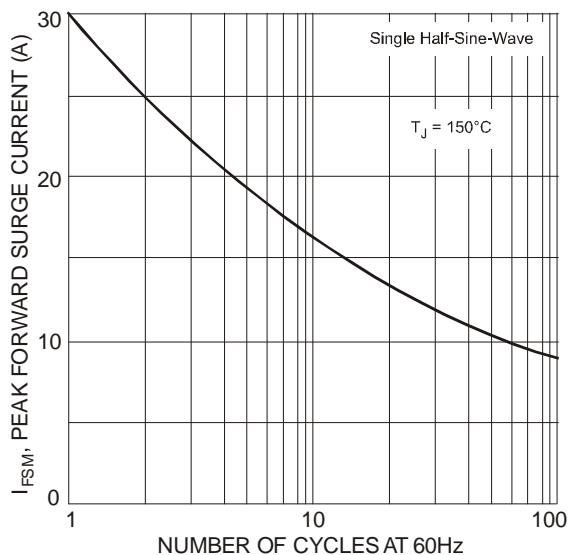
Fig. 4 Forward Surge Current Derating Curve
