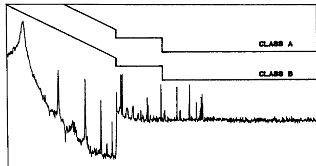
Fig. 4 Suppression effect of combined SN 223, RS 522, RN 114
