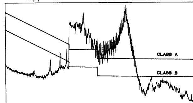
Fig. 2 Suppression effect of a RS 522-05
