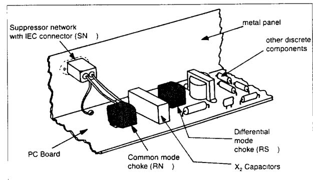
Fig. 3 A typical discrete filtering assembly
