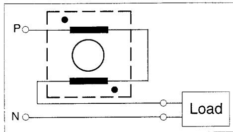
Functional schematic
