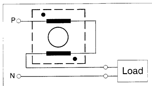
Functional schematic
