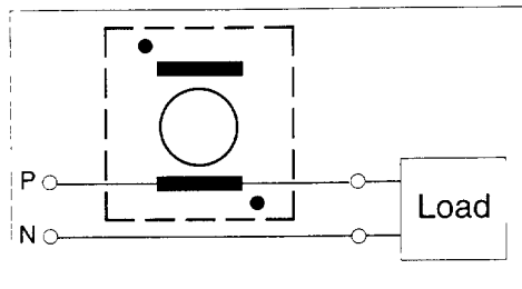
Functional schematic
