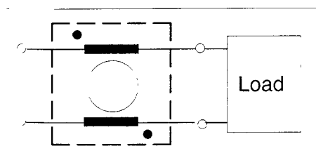
Functional schematic
