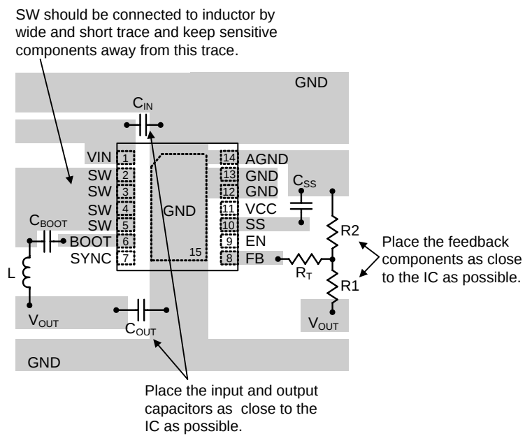
Figure 8. PCB Layout Guide
