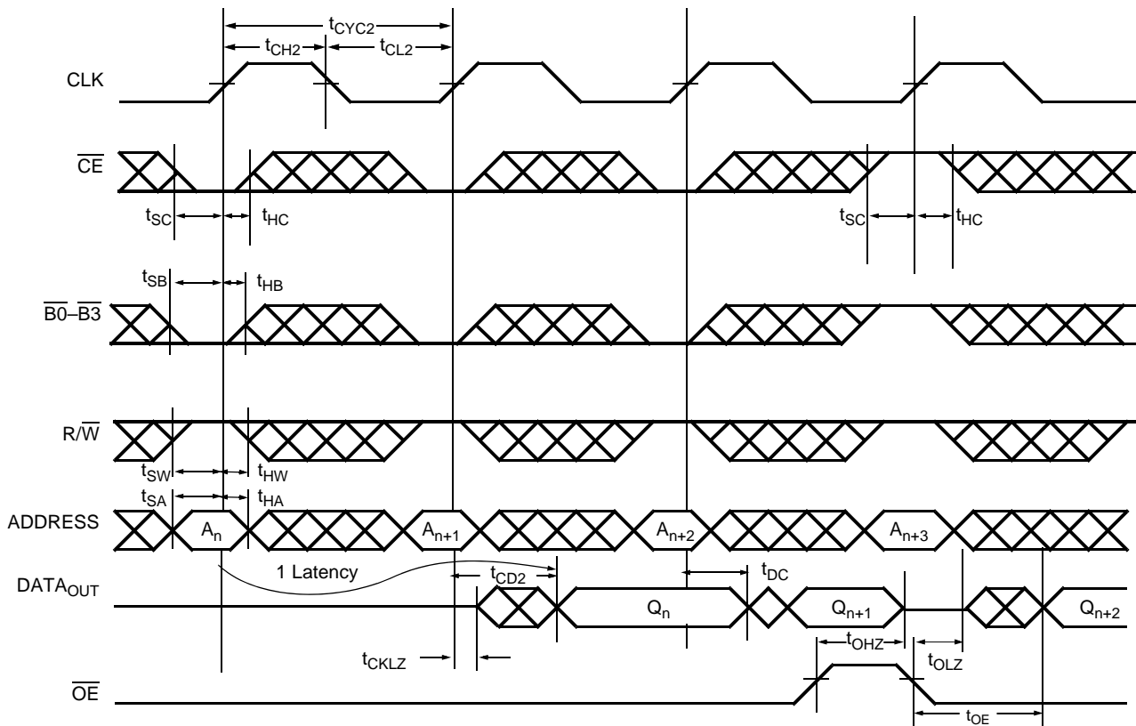
Figure 9. Read Cycle [32, 33, 34, 35, 36]
