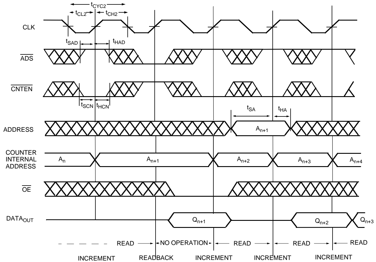
Figure 18. Read-to-Readback to Read-to-Read ( \overline{R/\overline{W}} = \text{HIGH} )
