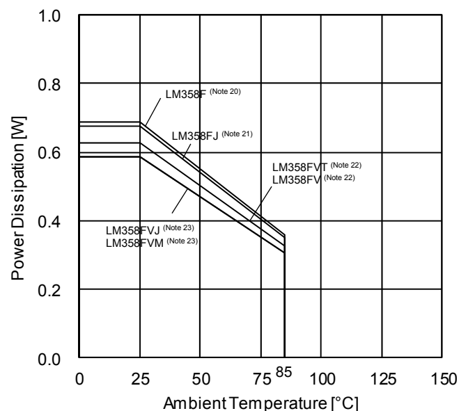
(c) LM358xxx
