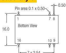
16 Pin SMD Package
