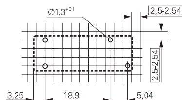
1 NO, 1 NC contact 5 mm
