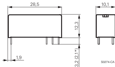
Pinning 5 mm
