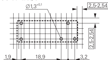
1 CO contact, 3.2 mm
