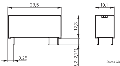
Pinning 5 mm
