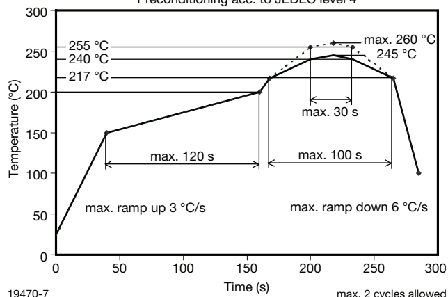
Fig. 18 - Vishay Lead (Pb)-free Reflow Soldering Profile (acc. to J-STD-020)
