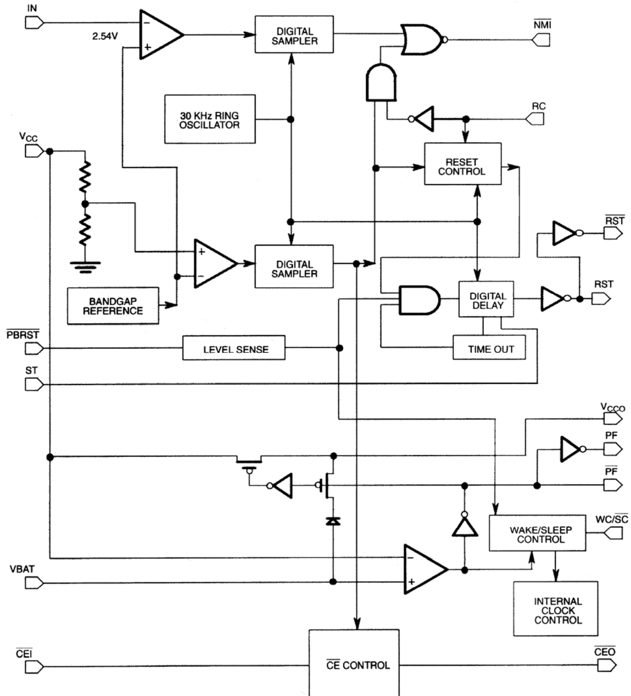
DS1236A FUNCTIONAL BLOCK DIAGRAM Figure 1
