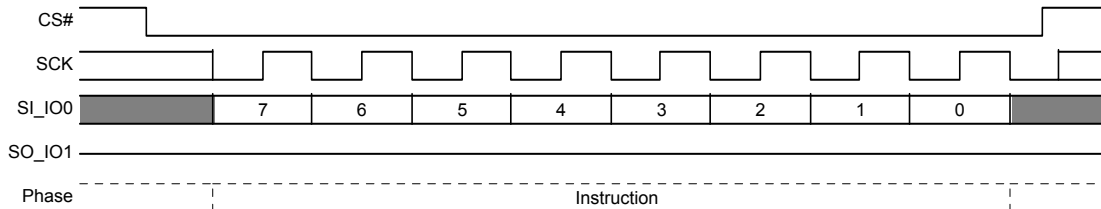
Figure 9.60 Chip Erase Command Sequence
