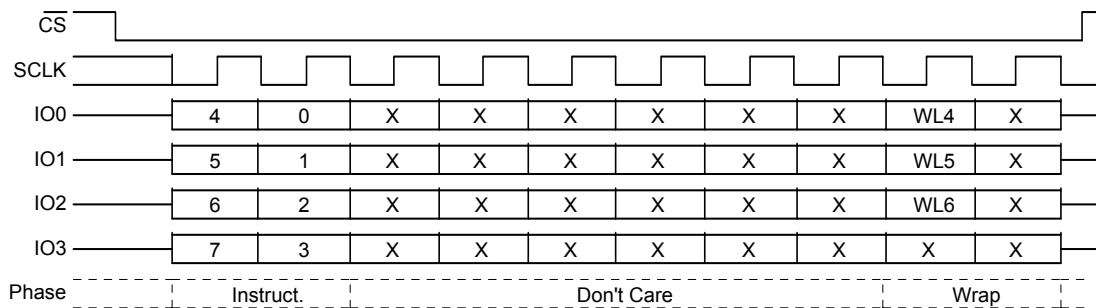
Figure 9.36 Set Burst Length Command Sequence QPI Mode
