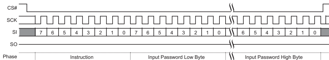
Figure 10.70 Password Program Command Sequence
