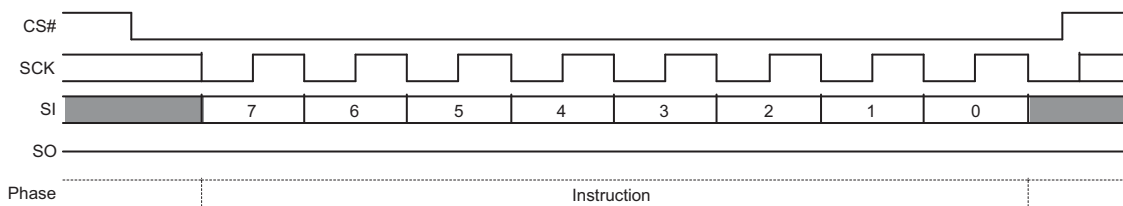
Figure 10.76 Deep Power-Down Command Sequence
