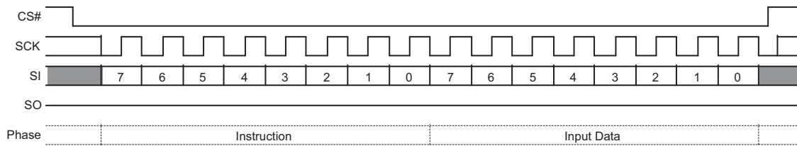
Figure 4.4 Single Bit Wide Input Command
