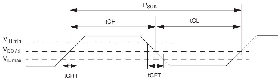
Figure 6.9 Clock Timing
