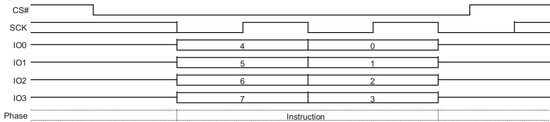
Figure 10.50 Bulk Erase Command Sequence QPI Mode
