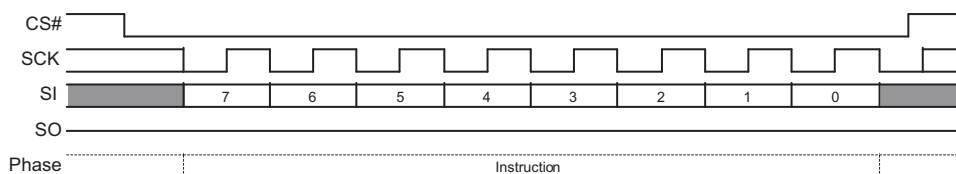
Figure 4.3 Stand Alone Instruction Command
