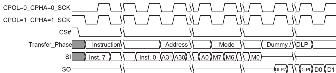
Figure 4.2 SPI DDR Modes Supported
