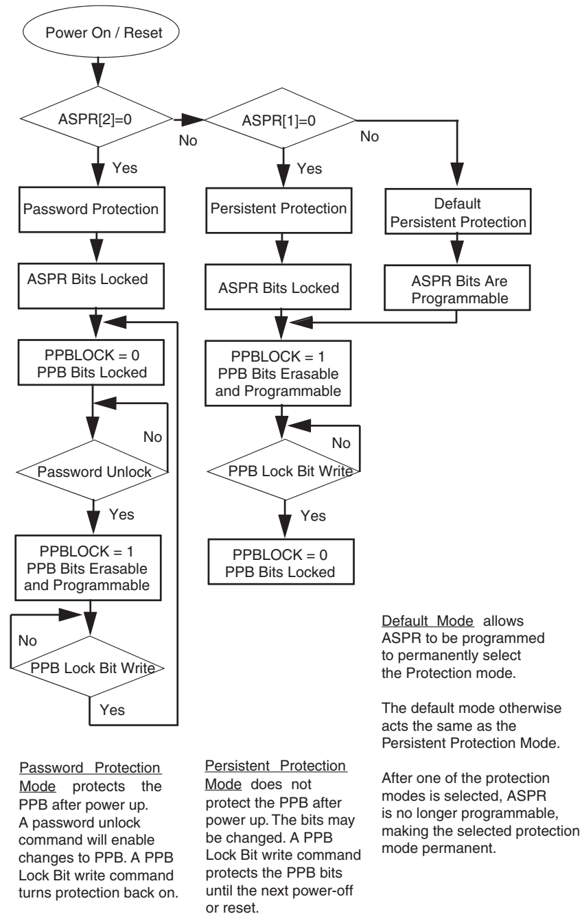
Figure 9.2 Advanced Sector Protection Overview
