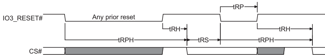
Figure 6.8 Hardware Reset when Quad Mode and IO3 / Reset# are Enabled
