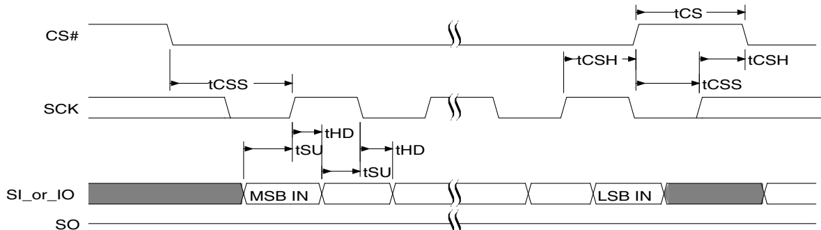
Figure 6.14 SPI DDR Input Timing
