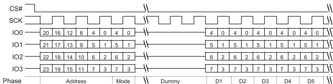
Figure 10.39 Continuous DDR Quad I/O Read Subsequent Access (3-Byte Address)
