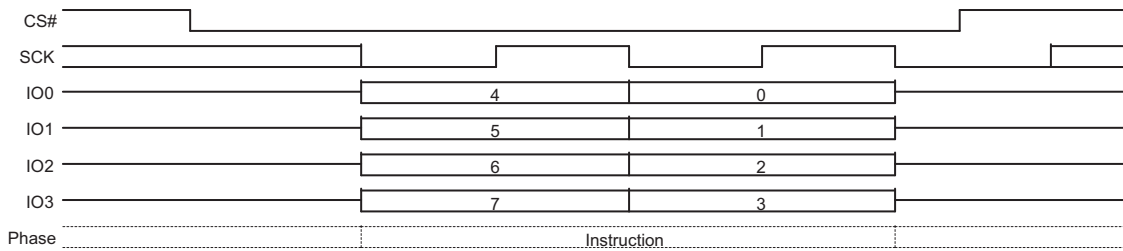
Figure 10.75 Mode Bit Reset Command Sequence QPI Mode
