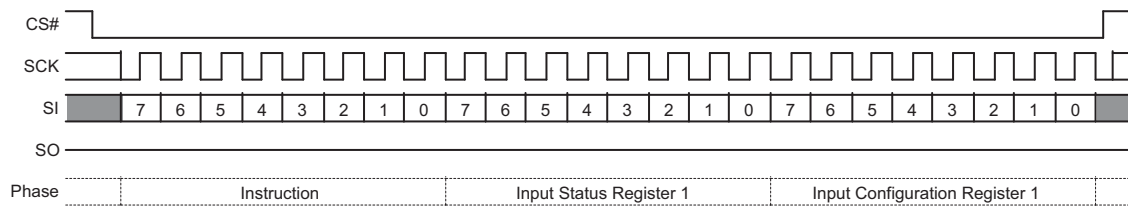
Figure 10.11 Write Registers (WRR) Command Sequence – 16-Data Bits
