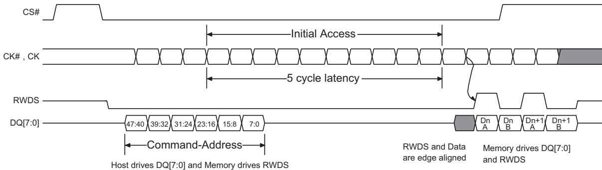
Figure 6. Read Operation
