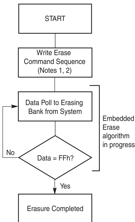
Figure 9.4 Erase Operation
