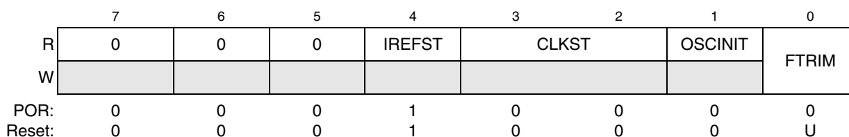
Figure 8-6. ICS Status and Control Register (ICSSC)
