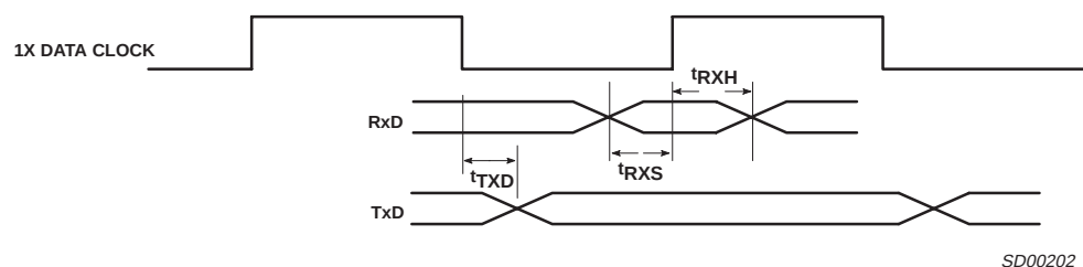
Figure 11. Transmitter and Receiver Timing
