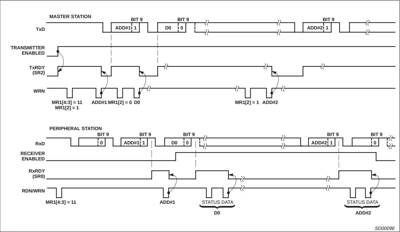
Figure 17. Wake-Up Mode
