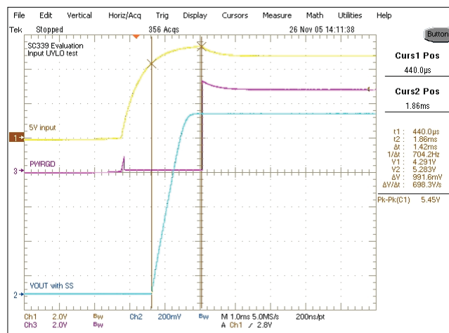
Figure 4: Input UVLO Test (Rising)
