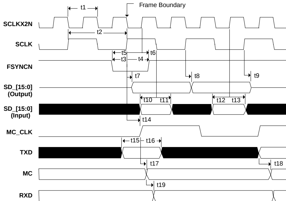
Figure 12. SCbus Timing
