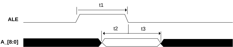
Figure 9. Microprocessor Interface Timing - Multiplexed Address
