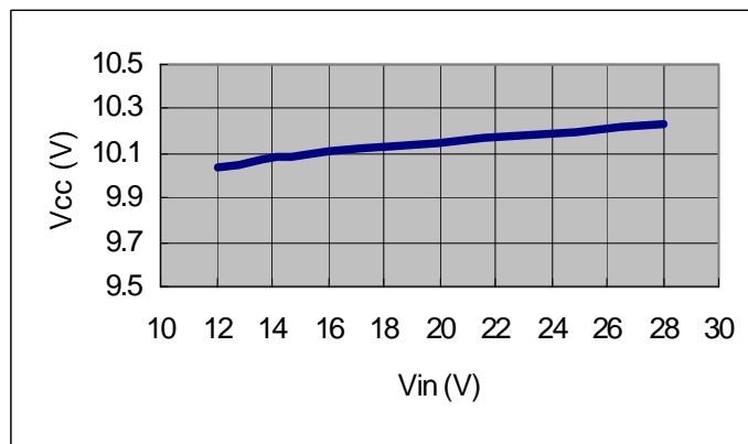
Vcc vs. Vin ( Ta=25 Degree C).
