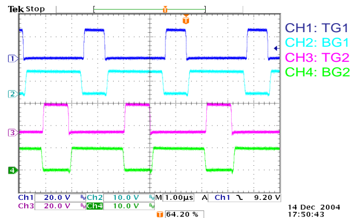
Gate waveform
