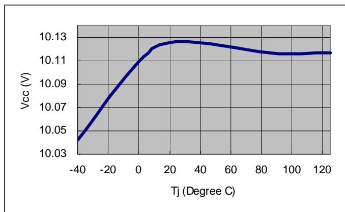
Vcc vs. Temp.
