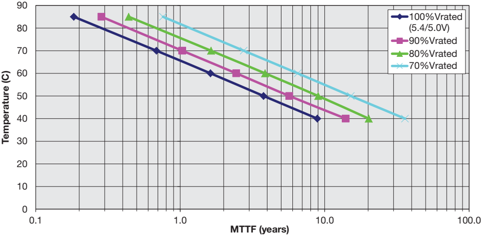
Expected Lifetime at Various Voltages SCM series 5.4/5.0V Rated
