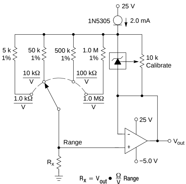
Figure 29. Linear Ohmmeter
