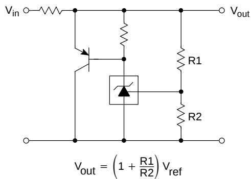
Figure 21. High Current Shunt Regulator
