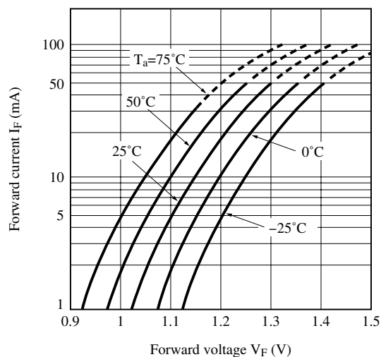
Fig.3-b Forward Current vs. Forward Voltage (Rank B, Rank C)
