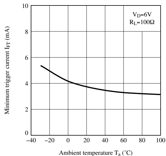
Fig.4-b Minimum Trigger Current vs. Ambient Temperature (Rank B, Rank C)
