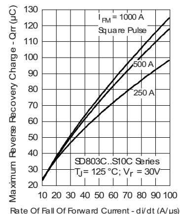
Fig. 12 - Recovery Charge Characteristics
