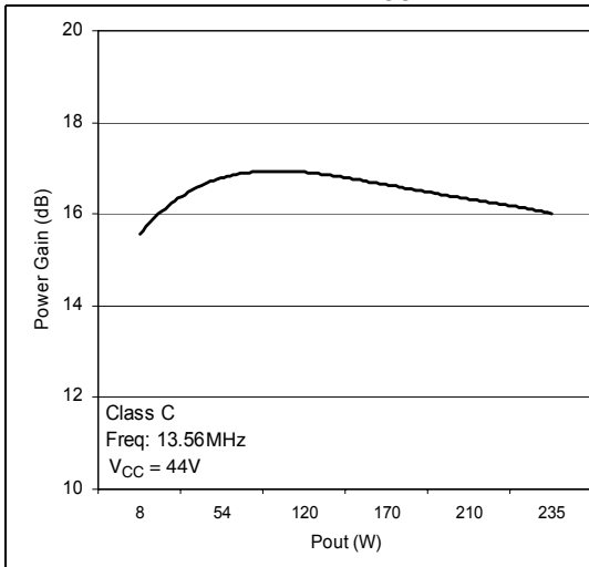
Figure 3. Power gain vs P_{OUT}
