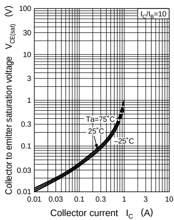
V_{CE(\text{sat})} - I_C
