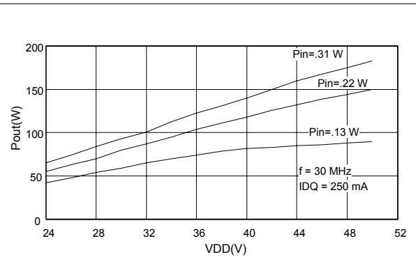
Figure 20. Output power vs supply voltage
