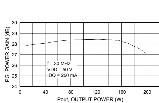
Figure 18. Power gain vs output power
