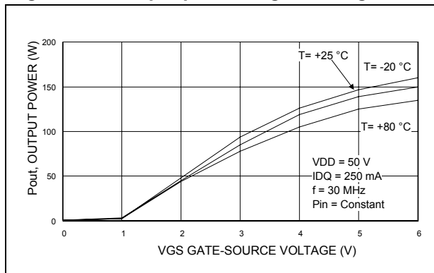
Figure 21. Output power vs gate voltage
