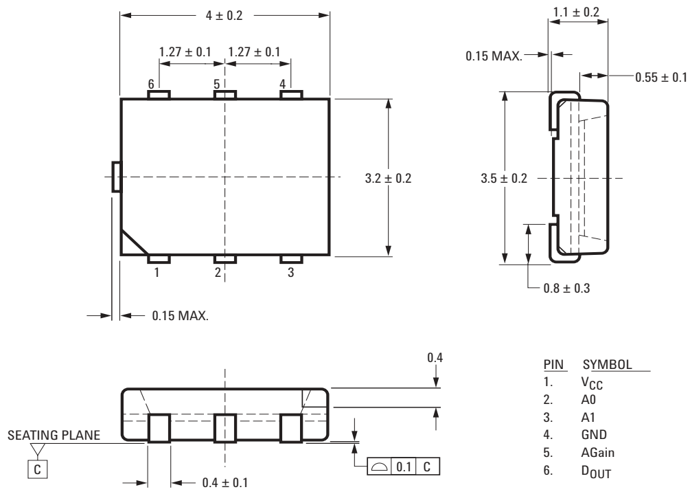
Figure 3. Package outline dimensions.
